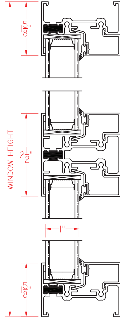
Ⓐ VERTICAL CROSS SECTION
