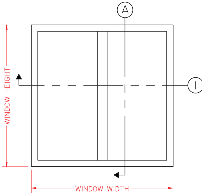
ELEVATION SCALE 3/4" = 1'-0"
