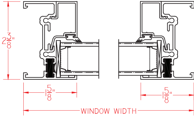
① HORIZONTAL CROSS SECTION
