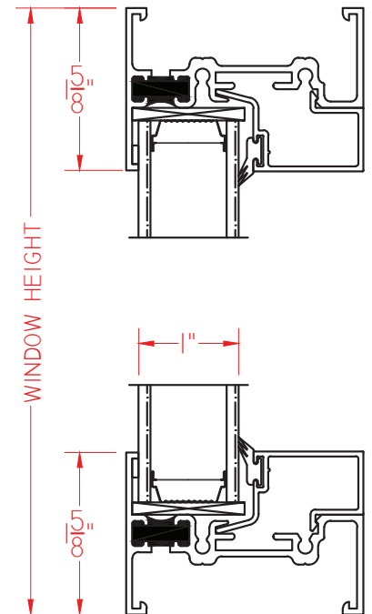
Ⓐ VERTICAL CROSS SECTION
