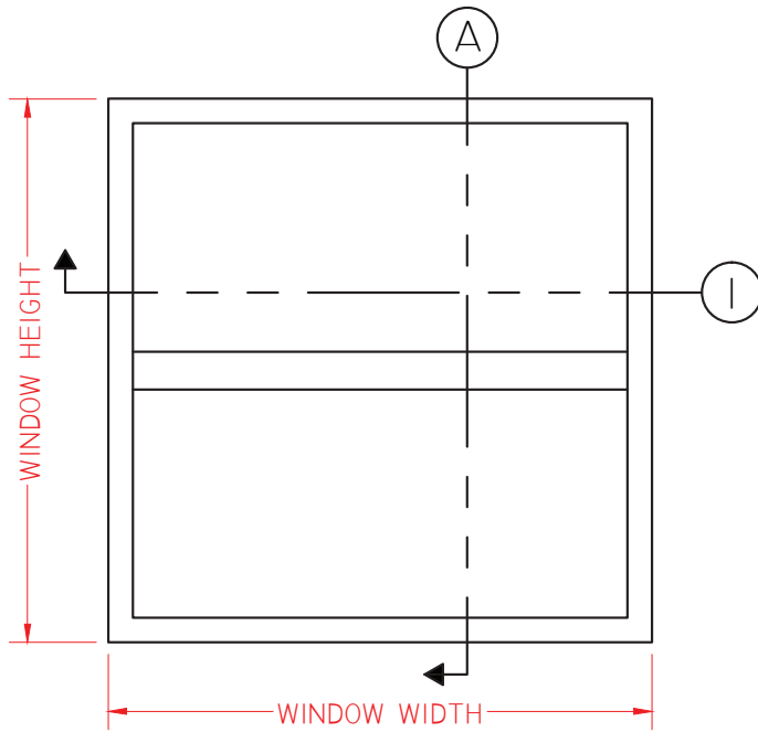
ELEVATION SCALE 3/4" = 1'-0"
