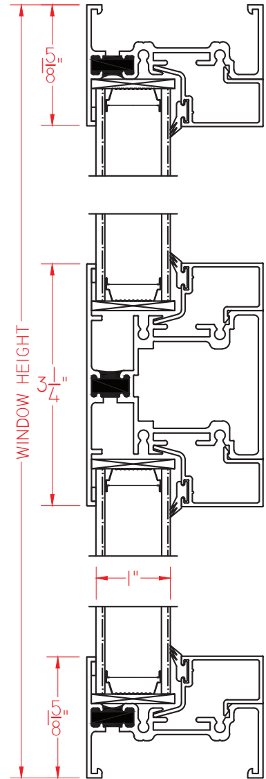
A VERTICAL CROSS SECTION
