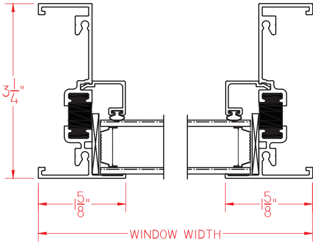
① HORIZONTAL CROSS SECTION
