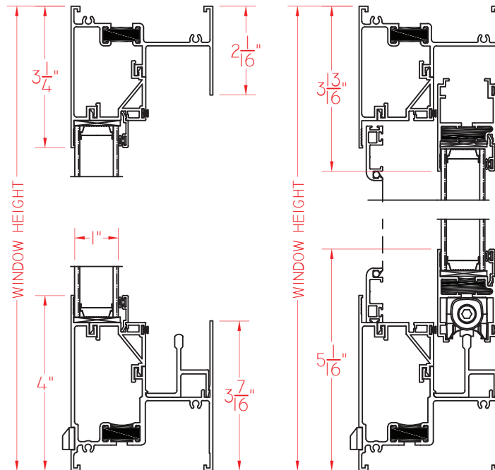
① A VERTICAL CROSS SECTION
