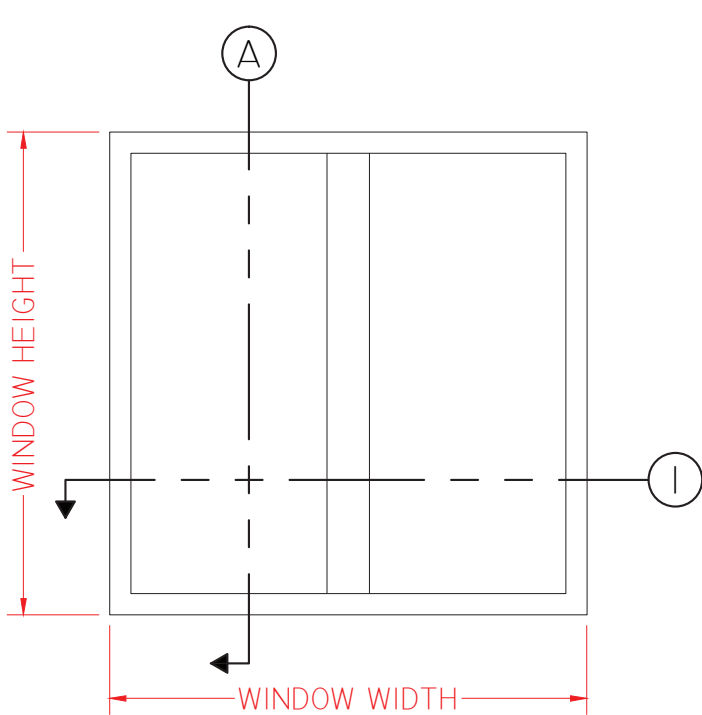
ELEVATION SCALE 3/4" = 1'-0"
