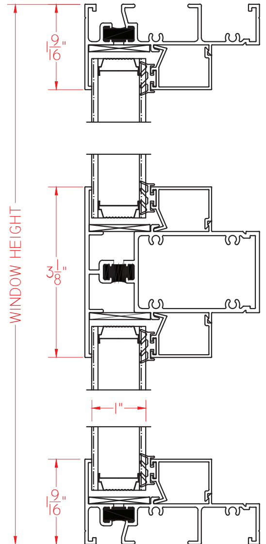
Ⓐ VERTICAL CROSS SECTION
