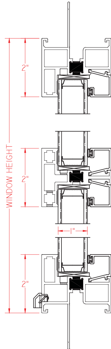
② VERTICAL CROSS SECTION
